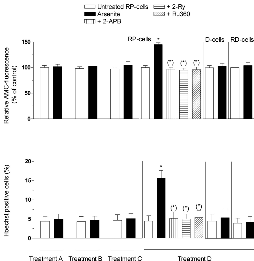
Fig. 6. Sustained increase in the [Ca^{2+}]_m leads to apoptosis. Cells were treated as indicated in the legend to Fig. 4, in which a definition of Treatment A-C is also provided. Treatment D refers to cells exposed to the metalloid for 48 h. RP-cells received Treatment D also in the presence of 2-APB, Ry or Ru360. After treatments, the cells were analyzed for caspase-3 activity (A), or for apoptosis, by measuring chromatin fragmentation/condensation with the Hoechst assay (B). Results represent the means \pm SD calculated from 5 separate experiments. * P < 0.01 , as compared to untreated cells. (*) P < 0.01 , as compared to cells treated with arsenite (one-way ANOVA followed by Dunnet's test).
