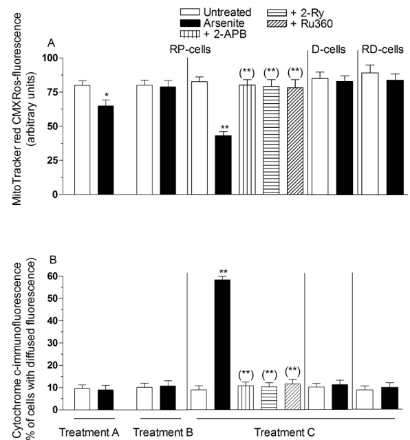
Fig. 5. Impact of transient vs sustained increase in the [Ca^{2+}]_m on mitochondrial dysfunction. Cells were treated as indicated in the legend to Fig. 4, in which a definition of Treatment A-C is also provided. RP-cells received Treatment C also in the presence of 2-APB, Ry or Ru360. After treatments, the cells were analyzed for MitoTracker red CMXRos-fluorescence (A) and cytochrome c localization (B), as detailed in the Methods section. Results represent the means \pm SD calculated from 4 to 6 separate experiments. * P < 0.05 , ** P < 0.01 , as compared to untreated cells. (**) P < 0.01 , as compared to cells treated with arsenite (one-way ANOVA followed by Dunnett's test).
