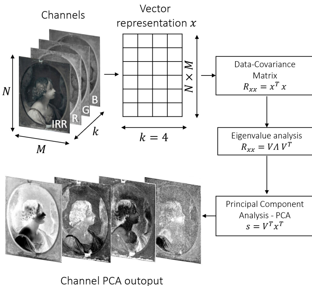
Figure 3.13 Scheme of Principal Component Analysis PCA applied to Image in visible light and multispectral.
