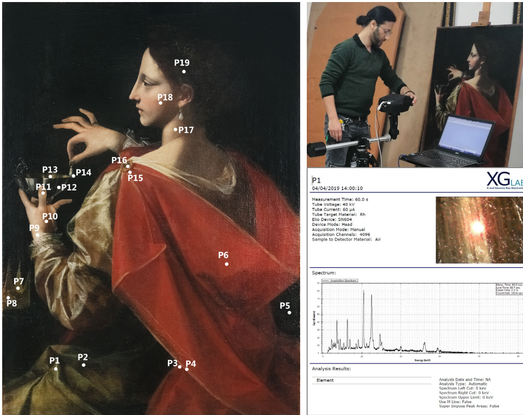
Figure 5.11: Points analyzed. Identification of measuring points with the XRF instrument. Performed by Stefano Pagnotta.
