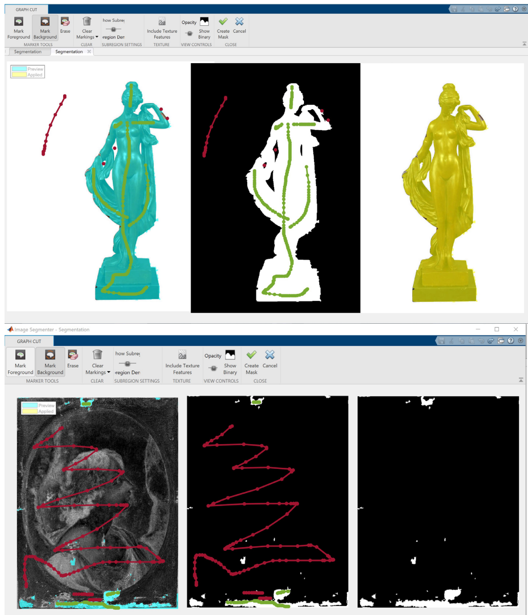
Figure 3.26 Matlab screenshot, Image Segmenter app. Example of segmentation using only the Graph cut tool. The more scribbles done, more the accuracy of the Graph Cut increases.
