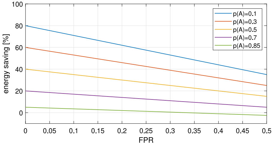
Fig. 2. Theoretical energy saved by the triggered approach with respect to the baseline when varying the FPR of the LAT classifier for different values of the probability p(A) .
