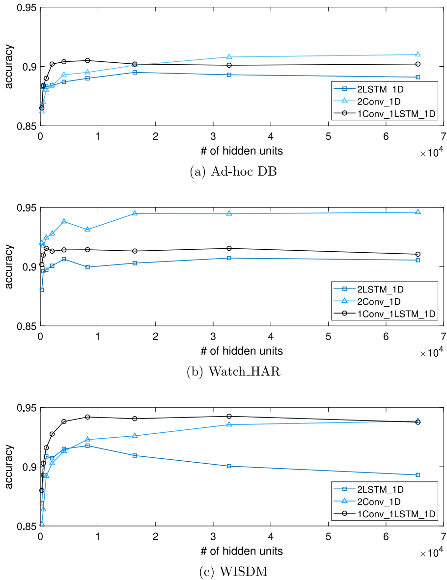
Fig. 7. Accuracy obtained by the proposed LAT models when varying the total number of hidden units on top of the three selected datasets.
