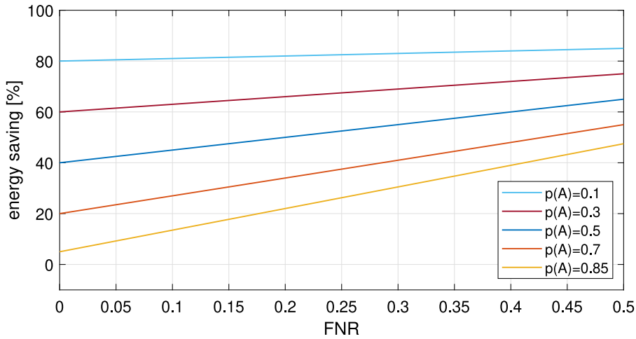
Fig. 3. Theoretical energy saved by the triggered approach with respect to the baseline when varying the FNR of the LAT classifier for different values of the probability p(A) .
