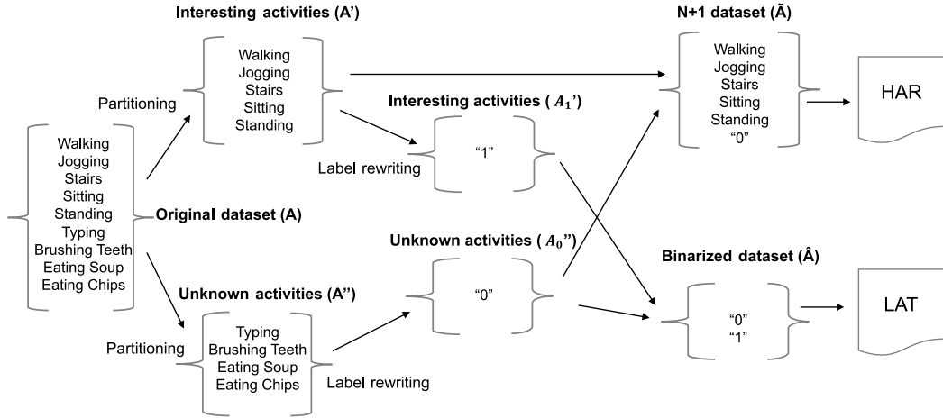
Fig. 4. The proposed workflow to train and test both LAT and HAR models starting from common HAR datasets.
