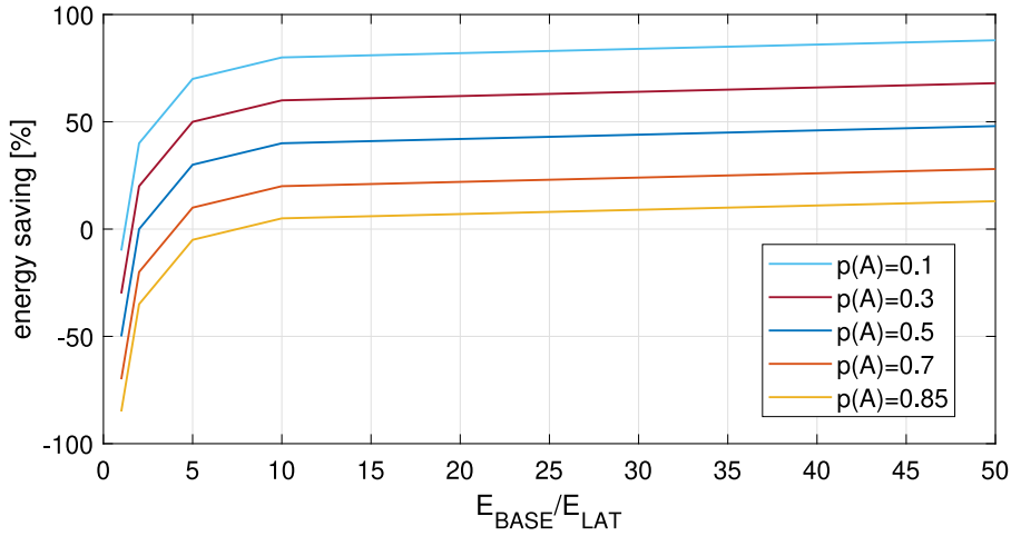
Fig. 1. Theoretical energy saved by the triggered approach with respect to the baseline (i.e. by using only the complete classifier) when varying the E_{BASE}/E_{LAT} ratio for different probability p(A) .
