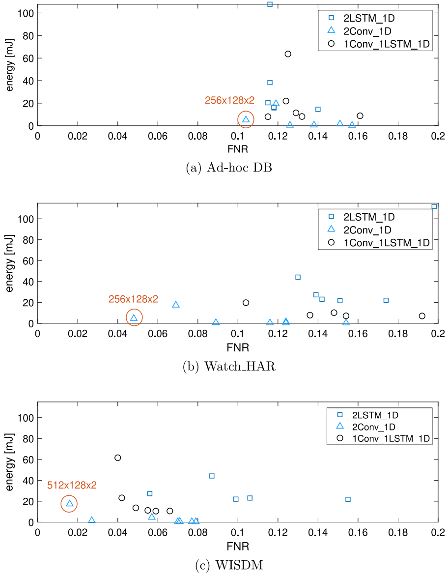
Fig. 8. Pareto diagram reporting the energy consumed in a single inference by each LAT configuration Vs its FNR.
