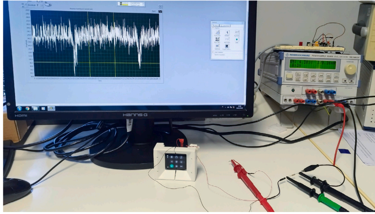
Fig. 6. The OPPO Watch 46 mm connected to the external power supply and to the measurement setup.
