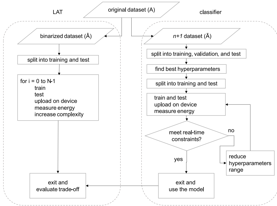
Fig. 5. The proposed workflow to build both the LATs and the complete models.
