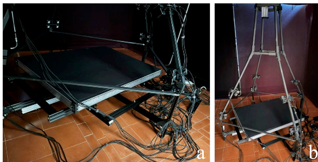
Figure 5. The elements of the horizontal repro stand: the lower frame (a) and the upper vertical frame (b).
