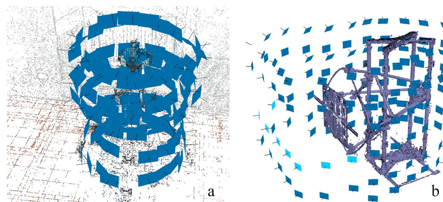
Figure 17. Radial camera network for the horizontal (a) and vertical (b) repro stands.
