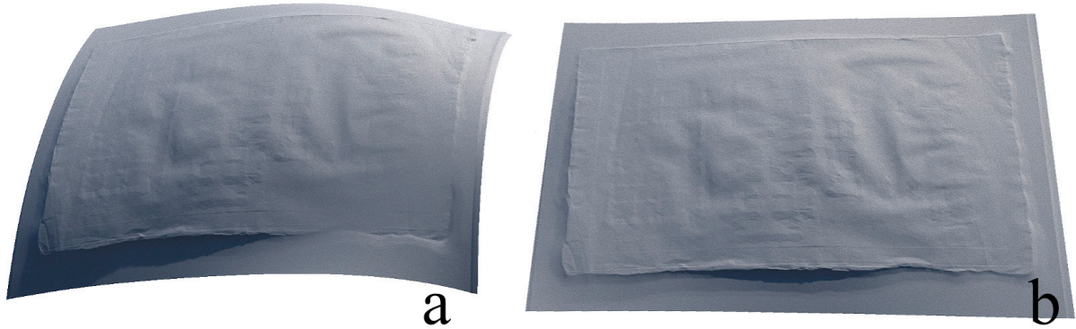
Figure 25. Comparison of the 3D meshes improved with the measured distances (b) and estimated ones (a); the typical “potato chip” effect is fixed. The vertical repro stand was adopted.
