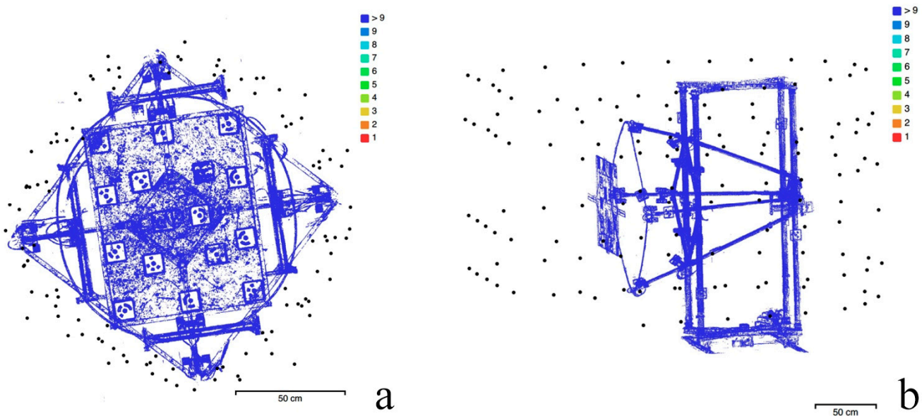
Figure 18. Shots coverage for the horizontal (a) and vertical (b) repro stands. Image alignment was performed with the open-source Colmap using images downsampled by a factor of 4 (two times for each side) and limiting the number of key points to 20,000.
