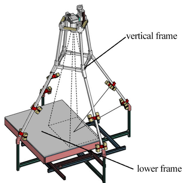
Figure 4. The horizontal repro stand.
