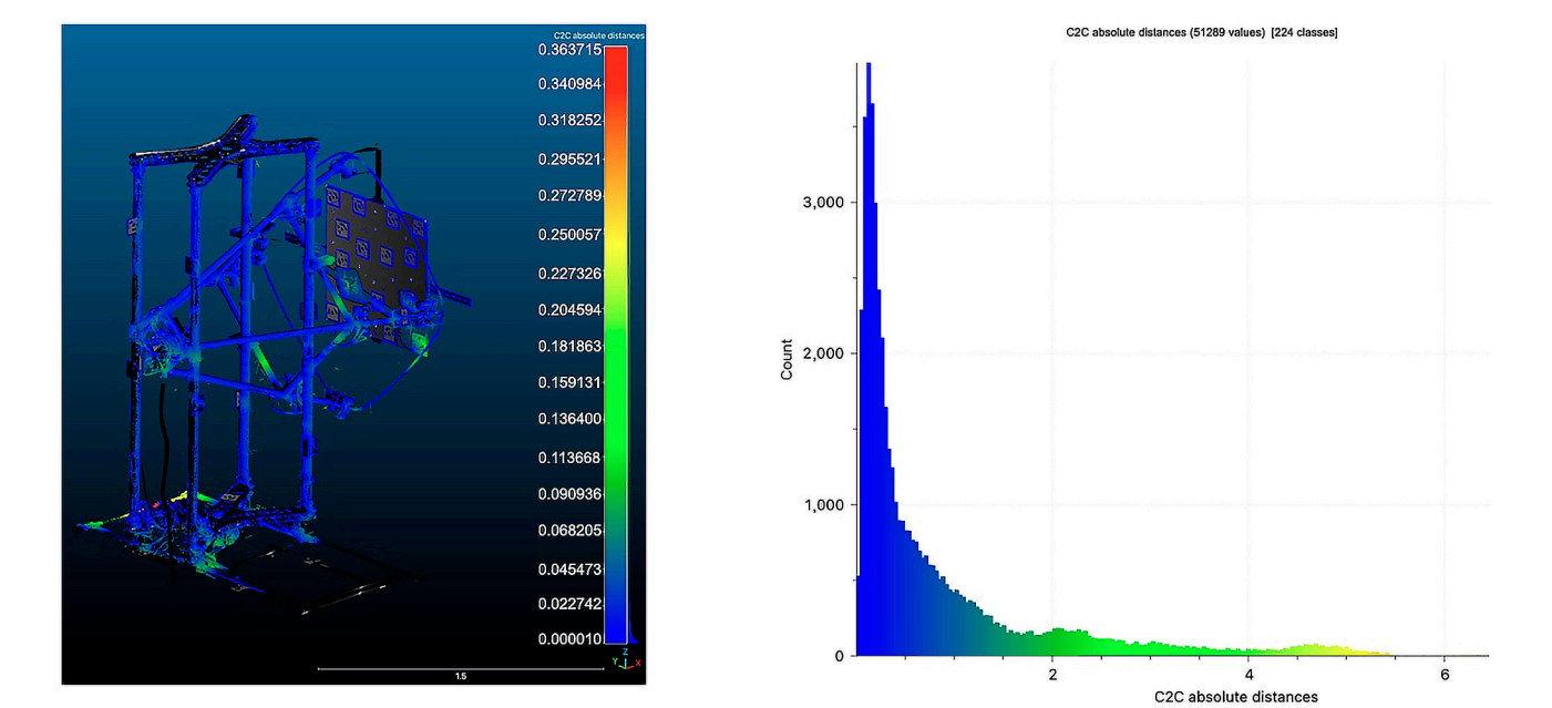
Figure 22. Point distribution errors of the cloud-to-cloud distances between ToF TLS system and photogrammetry (distances are in mm). Colors represented in the right graph correspond to those in the scale bar in the figure.
