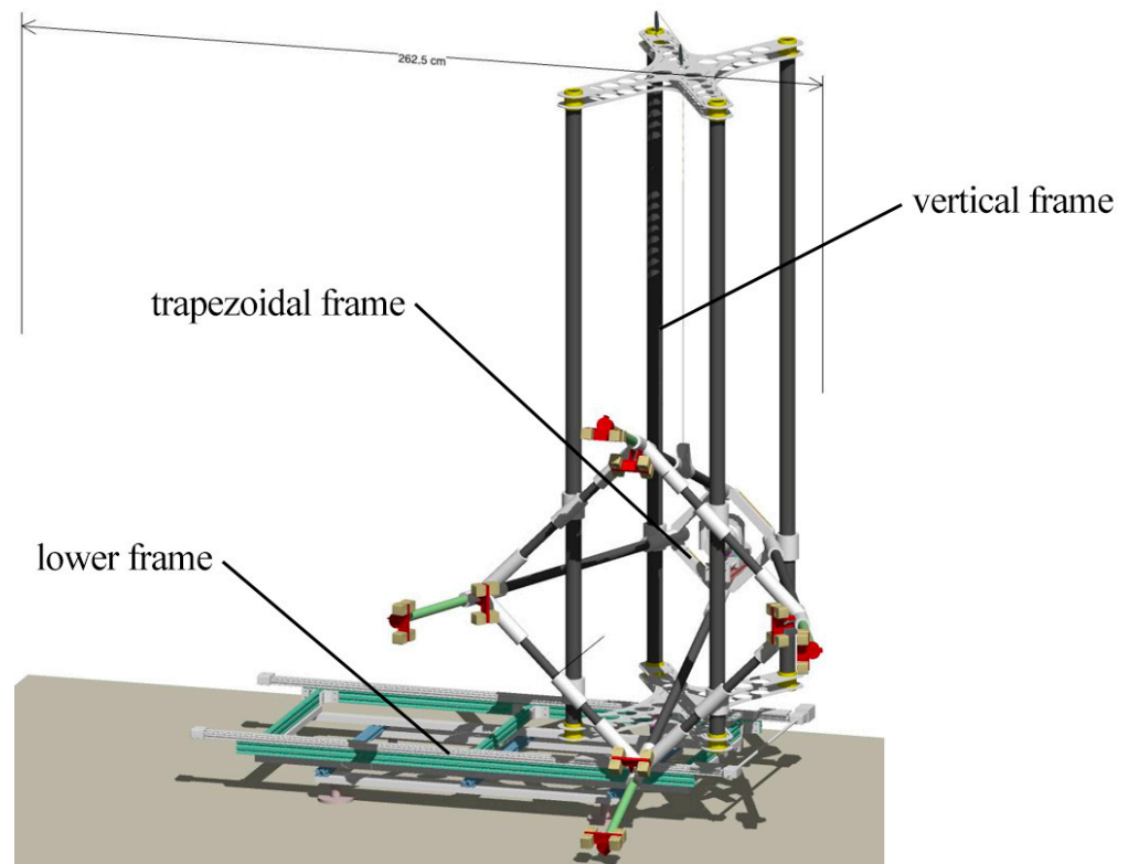
Figure 6. The robotized vertical repro stand and its components.
