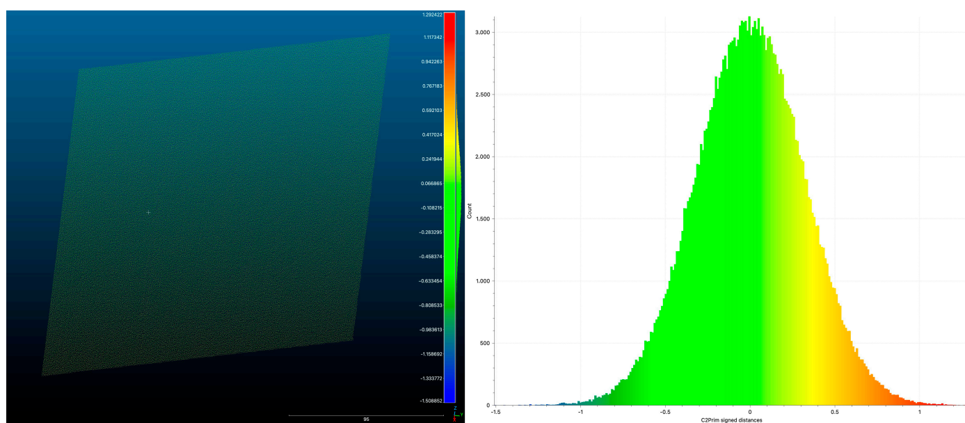
Figure 14. Point distribution errors of the cloud-to-fitting plane distances of the Leica RTC360 (distances are in mm). Colors represented in the right graph correspond to those in the scale bar on the figure.
