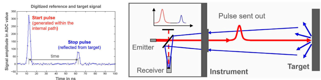
Figure 11. Schematics for WFD technology [91].
