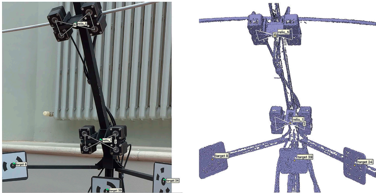
Figure 20. Pol identification through vector construction on dense cloud points.
