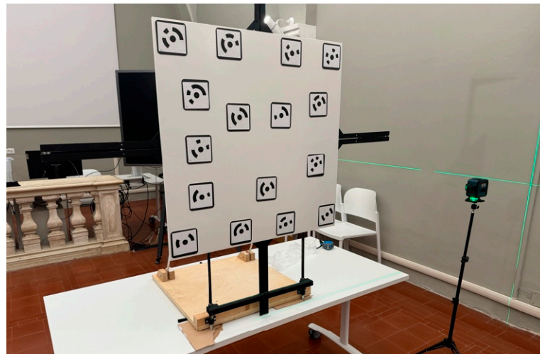
Figure 16. Vertical plane with the coded RAD targets.
