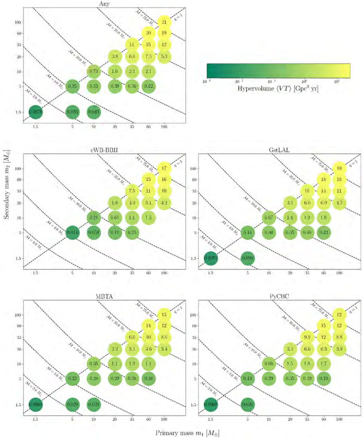
Figure 1. The sensitive hypervolume \langle VT \rangle for searches of O4a data applying a significance threshold \text{FAR} < 1 \text{ yr}^{-1} , evaluated at points in component mass space. The results labeled “Any,” presented in the upper left-hand panel, come from calculating the \langle VT \rangle for injections found by at least one search analysis. The color of each circle corresponds to the \langle VT \rangle value. The plotted points correspond to the central points of log-normal distributions with width 0.1 used to estimate \langle VT \rangle .
