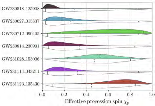
Figure 5. Posterior (upper, colored) and the effective prior (lower, white) probability distributions for the dimensionless effective precession spin \chi_p for candidates GW230518_125908, GW230627_015337, GW230712_090405, GW230814_230901, GW231028_153006, GW231114_043211, and GW231123_135430. Vertical lines mark the median and symmetric 90% interval for the distributions. These candidates are the ones that show the greatest deviation between the posterior distribution and the effective prior over the \chi_p parameter from the set of new candidates presented in this work.
