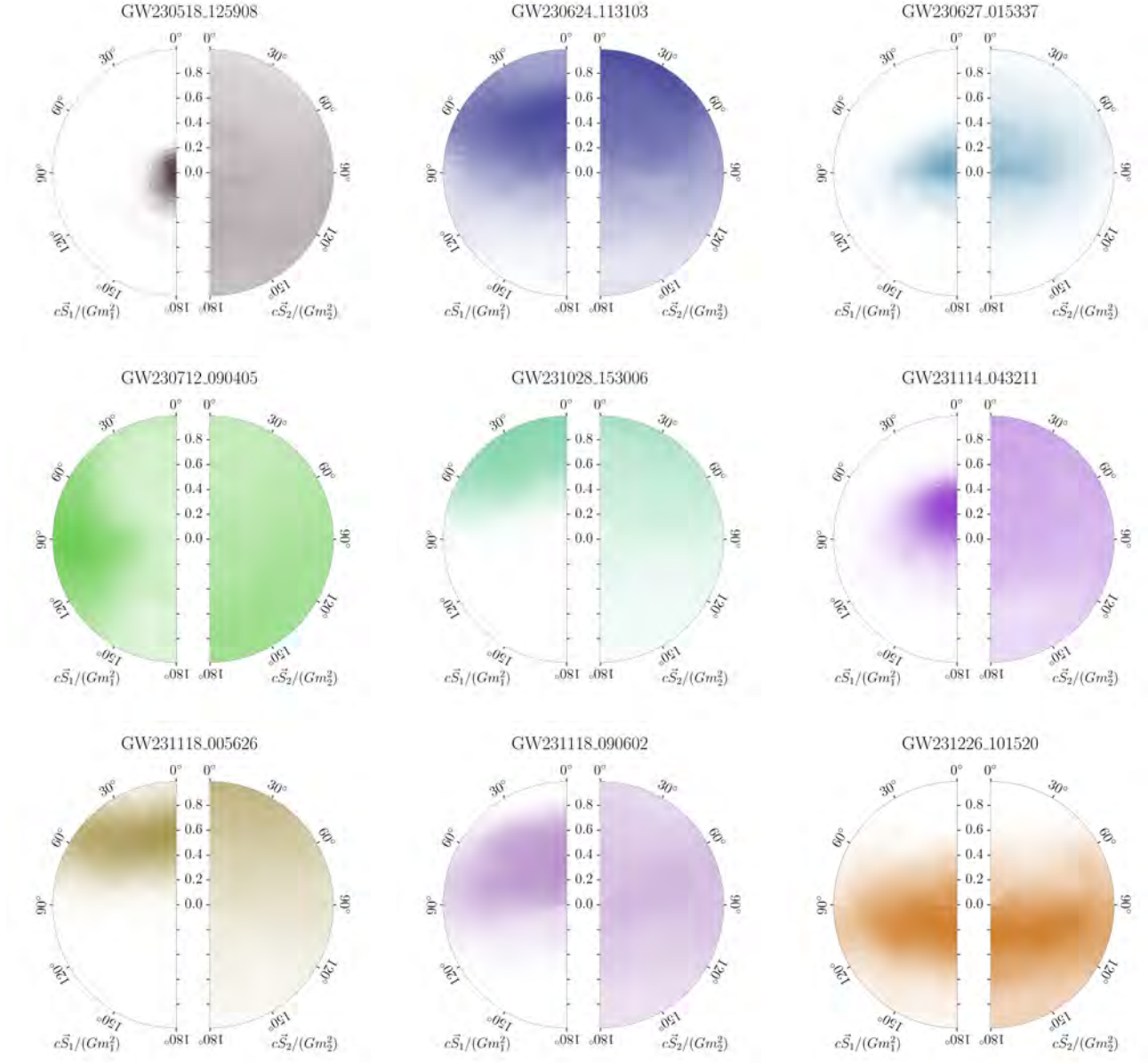
Figure 6. Posterior probability distributions for the dimensionless component spins \chi_1 = cS_1/(Gm_1^2) and \chi_2 = cS_2/(Gm_2^2) (with S_1 and S_2 the spin vectors of the components) relative to the orbital plane, marginalized over azimuthal angles, for candidates GW230518_125908, GW230624_113103, GW230627_015337, GW230712_090405, GW231028_153006, GW231114_043211, GW231118_005626, GW231118_090602, and GW231226_101520. In these plots, the histogram bins are constructed linearly in spin magnitude and the cosine of the tilt angles, such that they contain equal prior probability.
