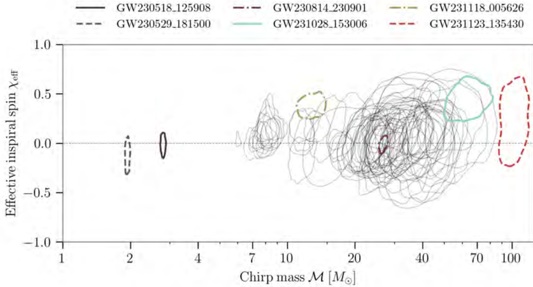
Figure 4. Credible-region contours in the chirp mass \mathcal{M} and effective inspiral spin \chi_{\text{eff}} plane for O4a candidates with FAR < 1 \text{ yr}^{-1} . Each contour indicates the 90% credible region for a given candidate. We use colors to highlight candidates GW230518_125908; GW230529_181500, which has an inferred \chi_{\text{eff}} < 0 at 92% credibility; GW231028_153006 and GW231118_005626, which have inferred \chi_{\text{eff}} > 0 ; GW230814_230901, which was the highest-SNR candidate observed in O4a; and GW231123_135430, which we infer to have the most massive source observed in O4a.
