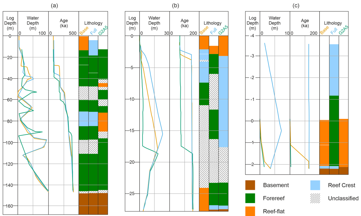
Figure 8. Dionisos model well logs for (a) Well A, (b) Well B, and (c) Well C. Water depth is depth of original deposition, age is time of deposition, and the dotted white lines represent unconformities. Line color corresponds to scenario: orange = Base, blue = Full, and green = G2A5.
