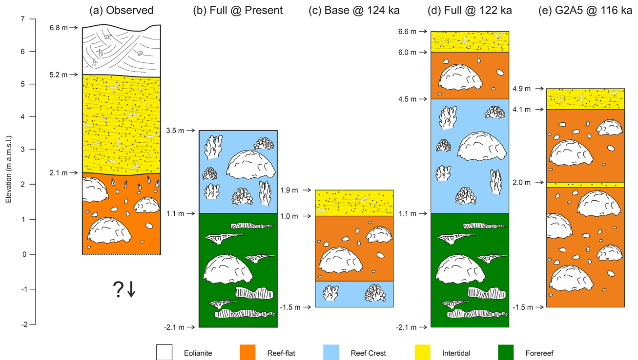
Figure 9. Comparison between field observations made by Boyden et al. (2022), lithology extracted from Full scenario at Well C at the end of the model run, and the lithologies for the Base, Full, and G2A5 scenarios at their highest respective MIS 5e unit before erosion takes place. (a) Synthesized litholog based on mean maximum facies elevations reported in Boyden et al. (2022). According to Boyden et al. (2022), the reef flat correlates to the MIS 5e highstand, the intertidal facies represents the close of MIS 5e, and the eolianite closes out the sequence correlating to much younger deposition. (b) Lithology at Well C for Full scenario at end of simulation. (c) Lithology at Well C for Baseline scenario at 124 ka when regression begins. (d) Lithology at Well C for Full scenario at 122 ka. (e) Lithology at Well C for G2A5 scenario at 116 ka. Colors represent the declared lithologies within the model environment and major bioconstructors are included for cross-comparison purposes.
