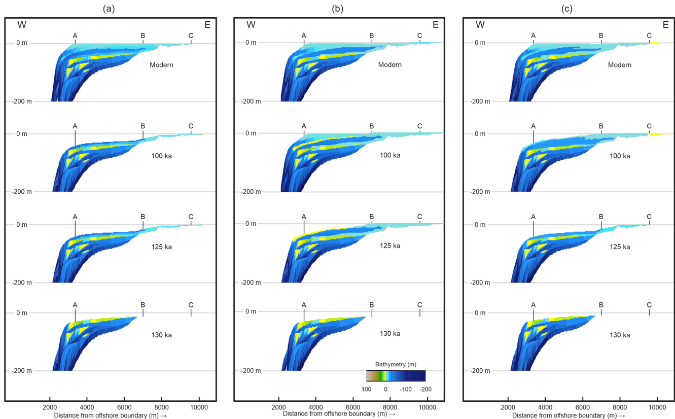
Figure 6. Dionisos model output for major event markers: 130 ka, 125 ka, 100 ka, and modern. (a) Baseline model driven by background GIA, (b) Full model incorporating simultaneous melting of GrIS and AIS, and (c) G2A5 model subjected to initial GrIS melting followed by AIS melting near the end of the LIG.
