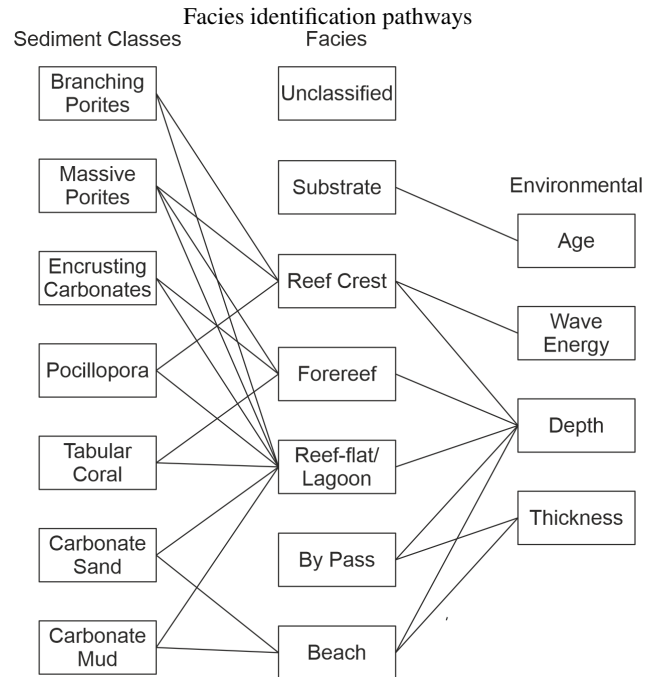
Figure 5. Identification pathways for determining facies within Dionisos. Adapted from Montaggioni (2005) and Seard et al. (2013).
