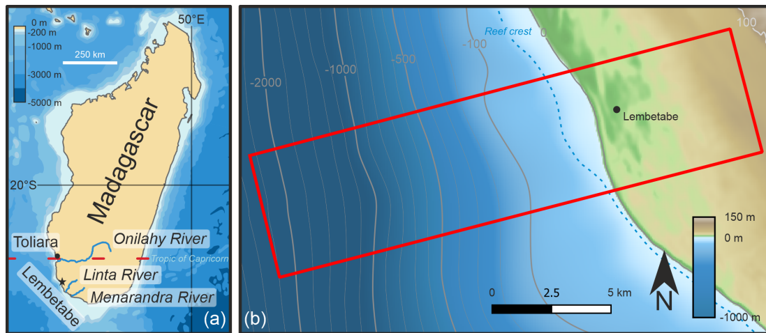
Figure 1. (a) Overview map of Madagascar, the study area at Lembetabe, and the three rivers in the southwest of the island. Map data from Natural Earth. (b) Overview of Dionisos model domain with combined topography/bathymetry detailed in Sect. 2.2.
