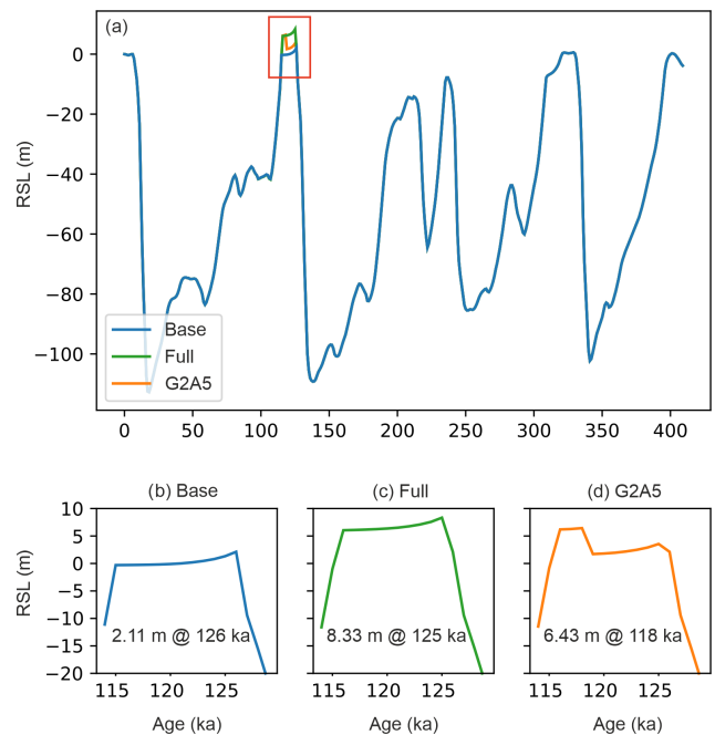
Figure 3. RSL sea level curves extracted from ANICE–SELEN for Lembetabe and used in Dionisos. (a) Overview of RSL over 400–0 ka. (b) Baseline curve with no further melting of GrIS or AIS beyond modern geometries at LIG. (c) Full RSL curve, with joint melting of GrIS (2 m) and AIS (5 m) at the onset of the LIG. (d) G2A5 RSL curve, with initial 2 m contribution from GrIS, followed by a later contribution of 5 m by AIS. Magnitude and timing of peak RSL in each scenario is included for reference.
