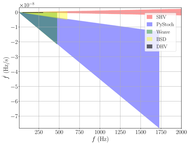
Figure 1. Parameter space covered by each of the five pipelines for G266.2 -1.2 (Vela Jr.).
