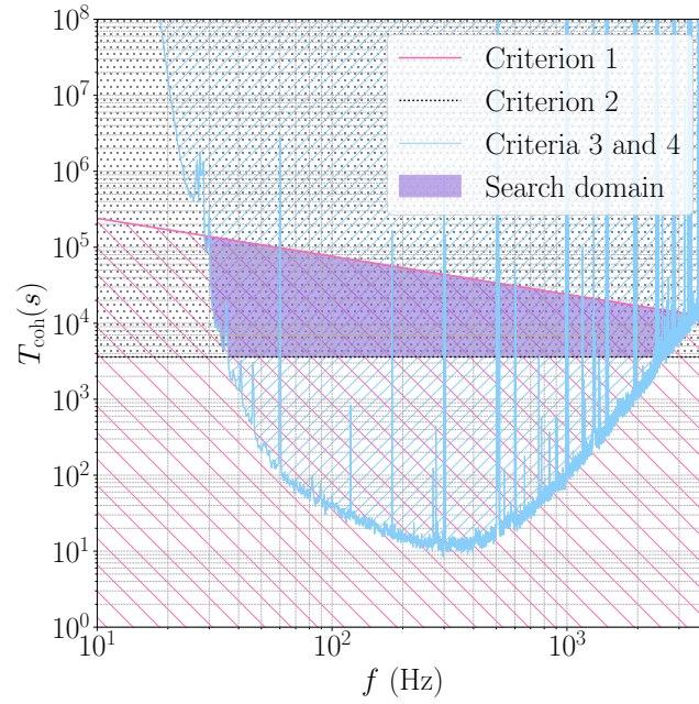
Figure 10. T_{\text{coh}} and f values that satisfy the four criteria defined in Appendix C.1.1. The shaded pink region satisfies criterion one, i.e., Equation (C3). The dotted gray region satisfies criterion two. The shaded blue region satisfies criteria three and four simultaneously. The purple domain indicates where all four criteria are satisfied, designated as the search region. For each f in the purple region, we choose T_{\text{coh}} according to the pink curve to maximize the search sensitivity.
