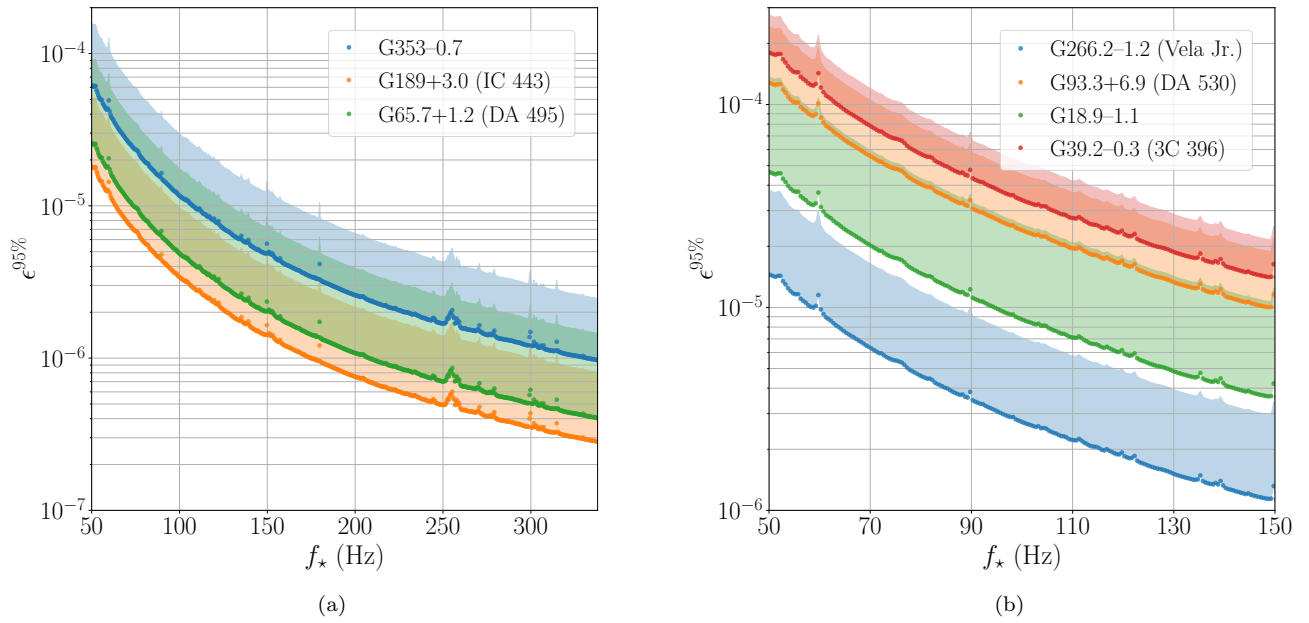
Figure 7. Constraints on the NS ellipticity with 95% confidence from the DHV search as a function of f_* for (a) T_{\text{coh}} = 12 hr and (b) T_{\text{coh}} = 9 hr, converted from the h_0^{95\%} values in Figure 12. The shaded region indicates the resulting ellipticity range calculated from the full estimated distance range for each SNR (see Table 1), and the solid dots correspond to the minimum distance estimate.
