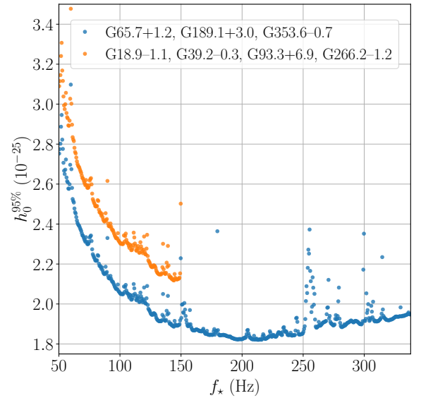
Figure 12. Estimated sensitivity h_0^{95\%} obtained from the DHV search as a function of f_{\star} for T_{\text{coh}} = 12 hr (blue) and T_{\text{coh}} = 9 hr (orange), assuming a specific scenario with source properties \theta = 45 deg and \cos i = 0 (signals at both f_{\star} and 2f_{\star} are linearly polarized). These estimates are obtained from randomized sky positions and hence apply to all sources using the same T_{\text{coh}} .
