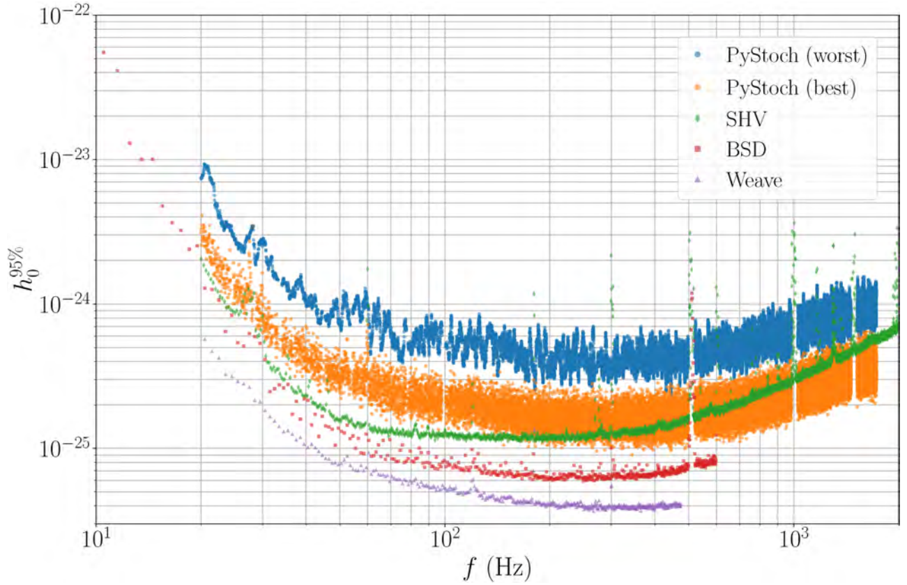
Figure 2. Upper Limits for the source G266.2–1.2 (Vela Jr.) obtained for the pipelines assuming the single-harmonic emission scenario. The dual-harmonic results for the same source are shown in Figure 12.
