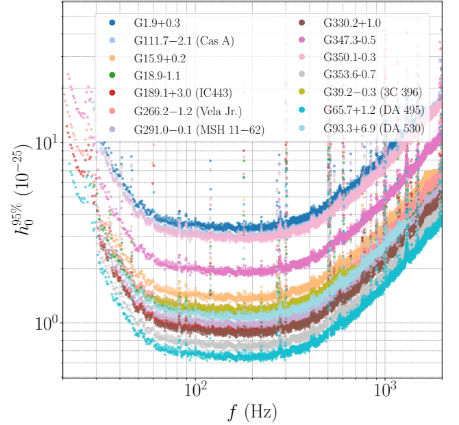
Figure 11. Upper-limit curves for all targets searched by the SHV pipeline. The scatter points show the sensitivity estimate h_0^{95\%}(T_{\text{coh}}) = a(T_{\text{coh}})h_0^{\text{est}} across the searched frequency band.
