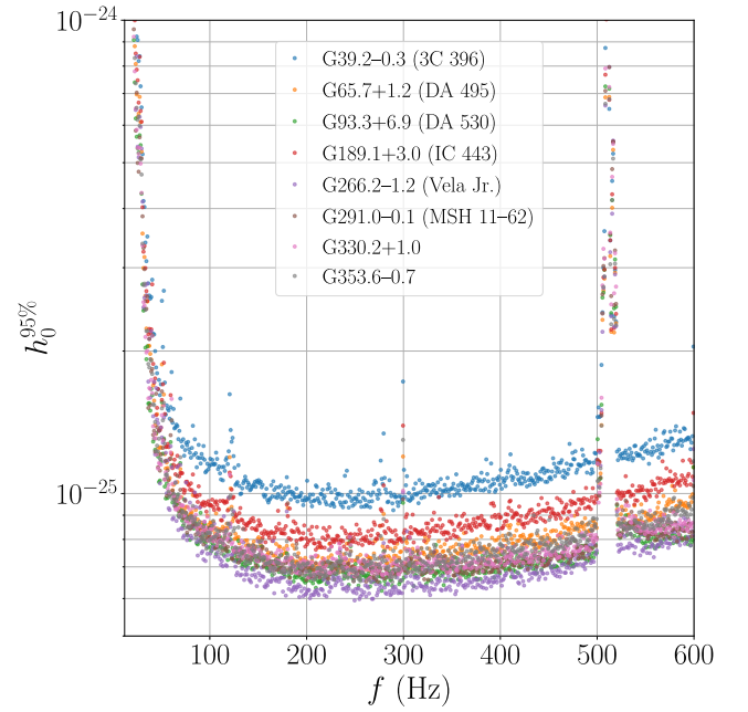
Figure 8. Estimated 95% confidence-level upper limit obtained from the BSD search.
