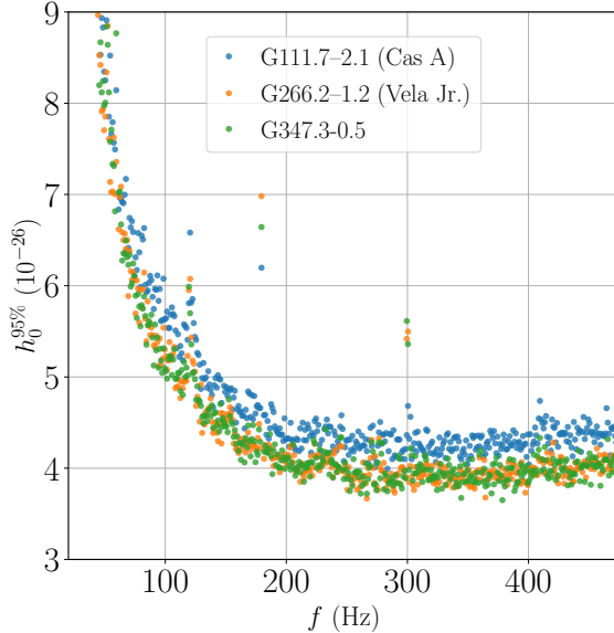
Figure 13. GW strain amplitude upper limits (95% confidence level) in each 1 Hz band for the Cas A (blue), Vela Jr. (orange), and G347.3–0.5 (green) searches using Weave. All the upper limits presented here are below the age-based strain amplitude limit ( >10^{-24} ) for the three targets.
