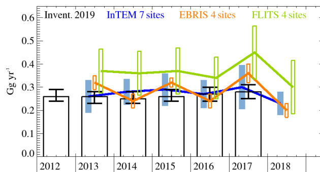
Figure 6. SF 6 western Europe emission estimates (Gg yr -1 ) from the UNFCCC inventory (black); InTEM inversion (2013–2018, blue, seven sites: MHD, JFJ, CMN, TAC, RGL, HFD, BSD); EBRIS (2013–2018, orange, 4 sites: MHD, TAC, JFJ, CMN); and FLITS (2013–2018, green, four sites: MHD, TAC, JFJ, CMN). The uncertainty bars are \pm 1 SD.
