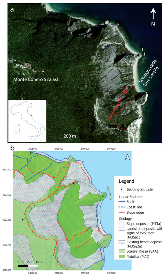
Fig. 1 - a) Study area with highlighted the Passo del Lupo trail (red line) and the Spiaggia delle due Sorelle beach. B) Geological map of the study area
