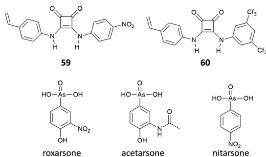
Fig. 22 Squaramides 59 and 60 used to prepare MIPs for the solid-state extraction of the organoarsenic compound roxarsone. The structures of roxarsone analogues acetarsone and nitarosone are also reported.
