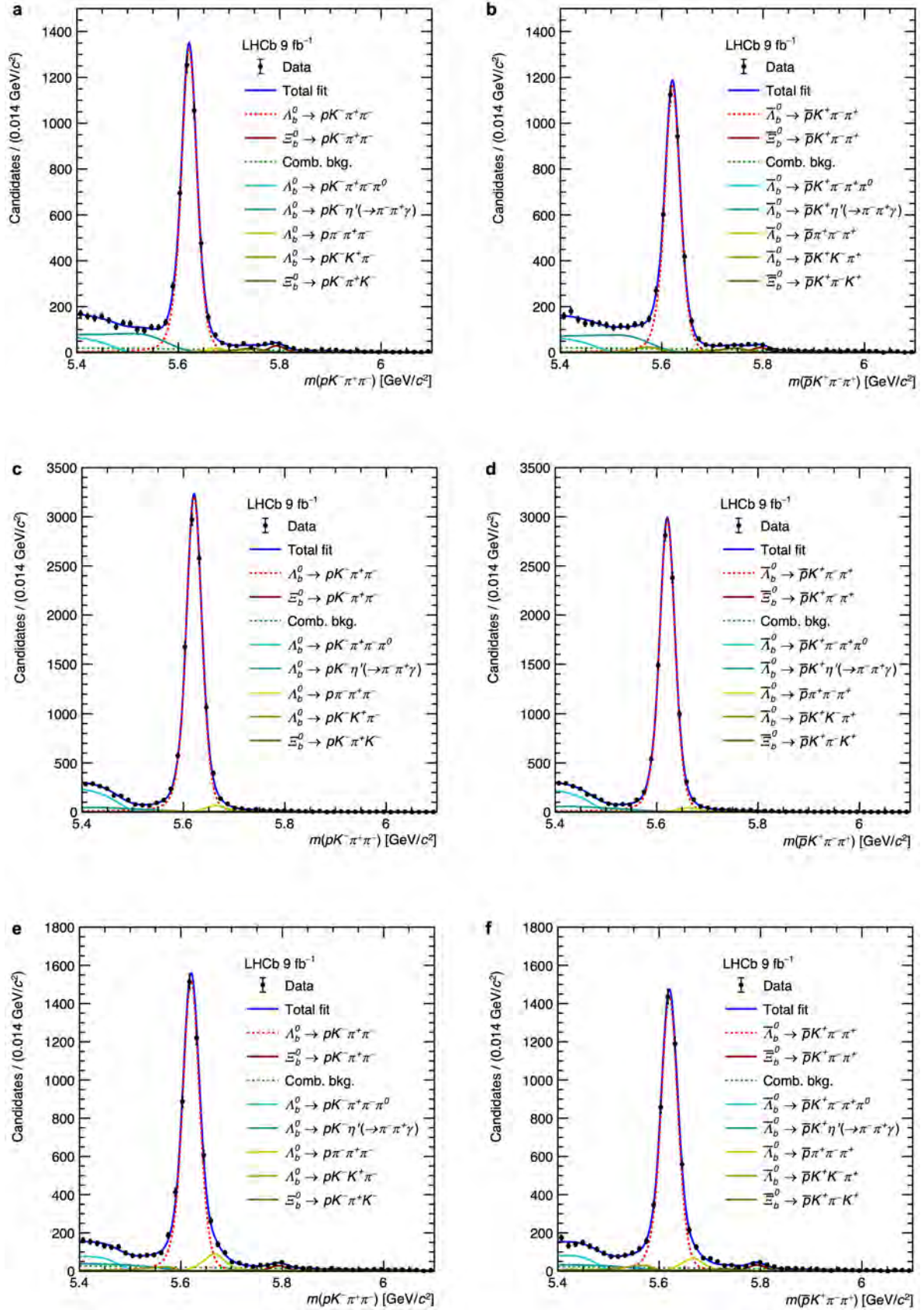
Extended Data Fig. 3 | Mass distributions in regions of phase space with the fit projections also shown. Mass distributions of \Lambda_b^0 \rightarrow pK^- \pi^+ \pi^- and \Lambda_b^0 \rightarrow \bar{p}K^+ \pi^- \pi^+ for (a, b) \Lambda_b^0 \rightarrow R(pK^-)R(\pi^+ \pi^-) , (c, d) \Lambda_b^0 \rightarrow R(p\pi^-)R(\pi^+ K^-) , and (e, f) \Lambda_b^0 \rightarrow R(K^- \pi^+ \pi^-)p decays.
